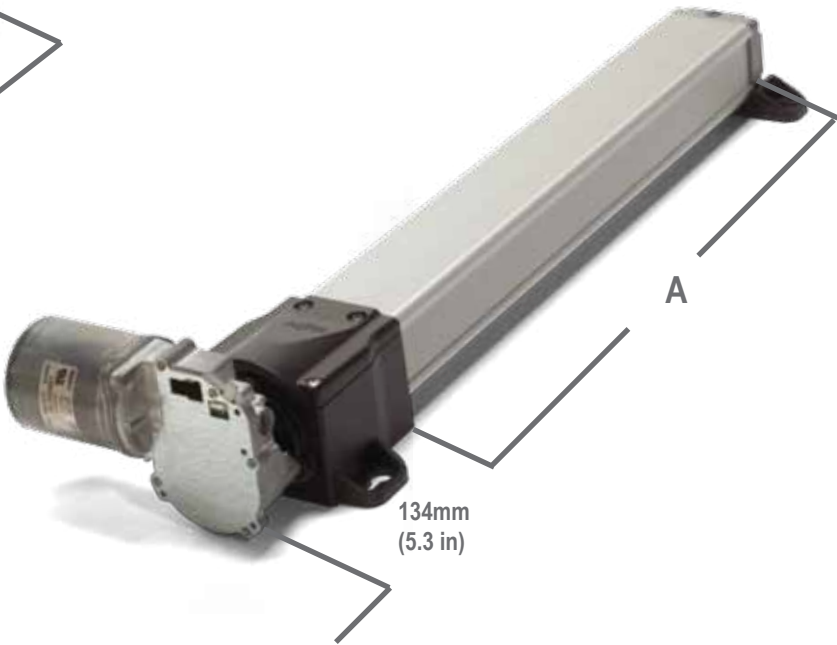
Motor Driven
